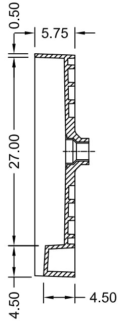
SECTION B-B
